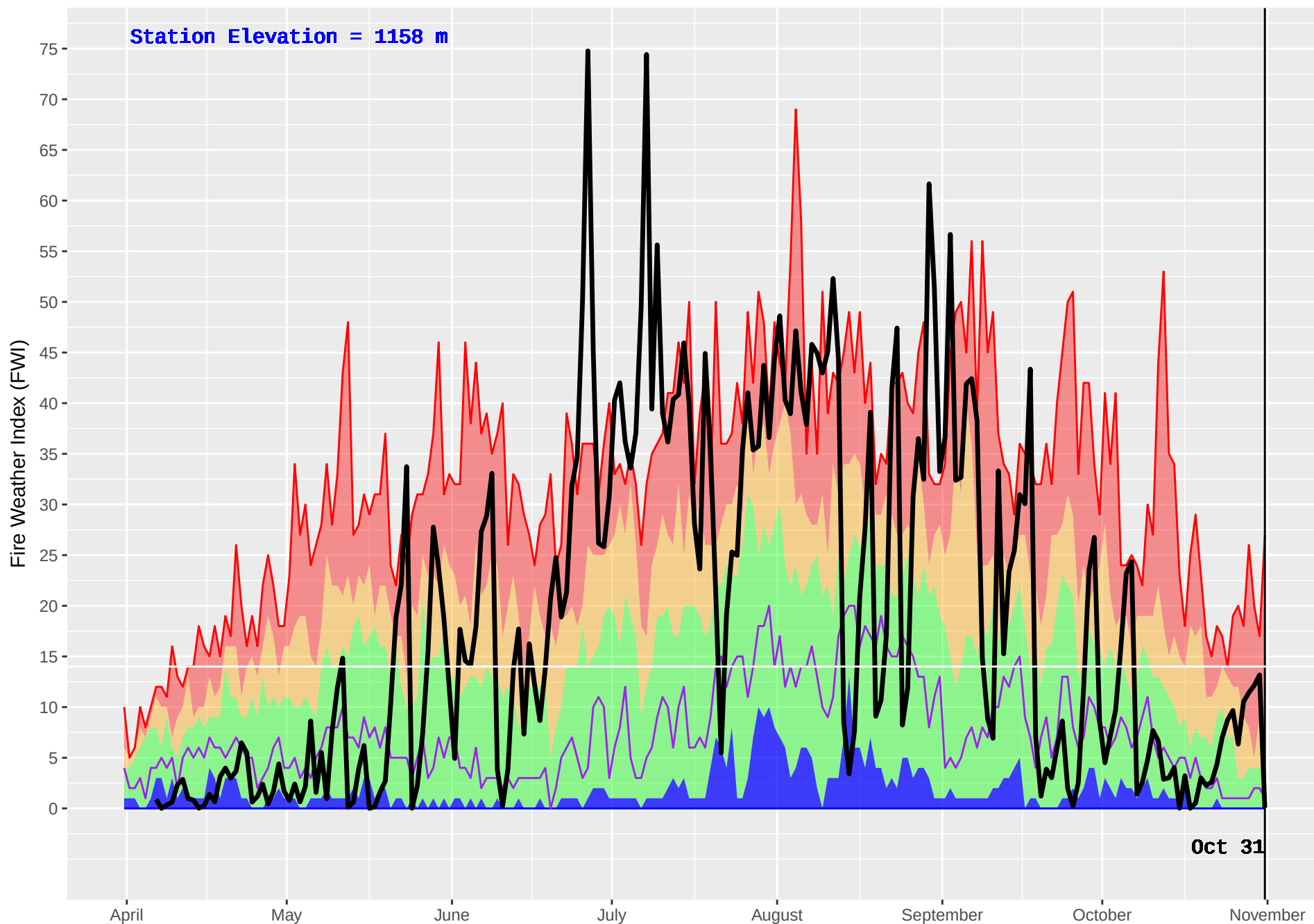
LONE BUTTE (218) : Historical (1987–2016) and Current (2017) Noon Fire Weather Index (FWI)
