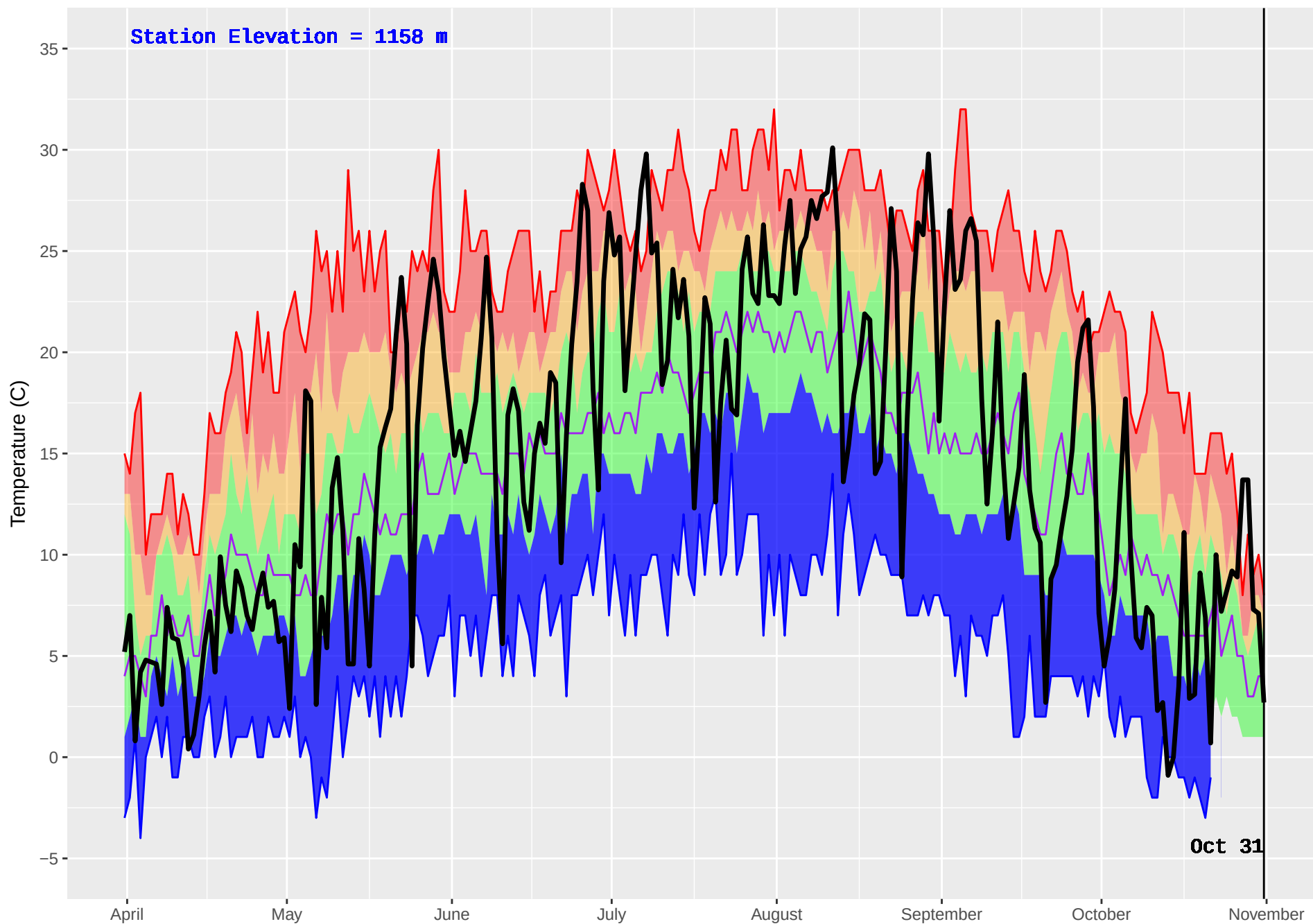
LONE BUTTE (218) : Historical (1987–2016) and Current (2017) Noon Temperature
