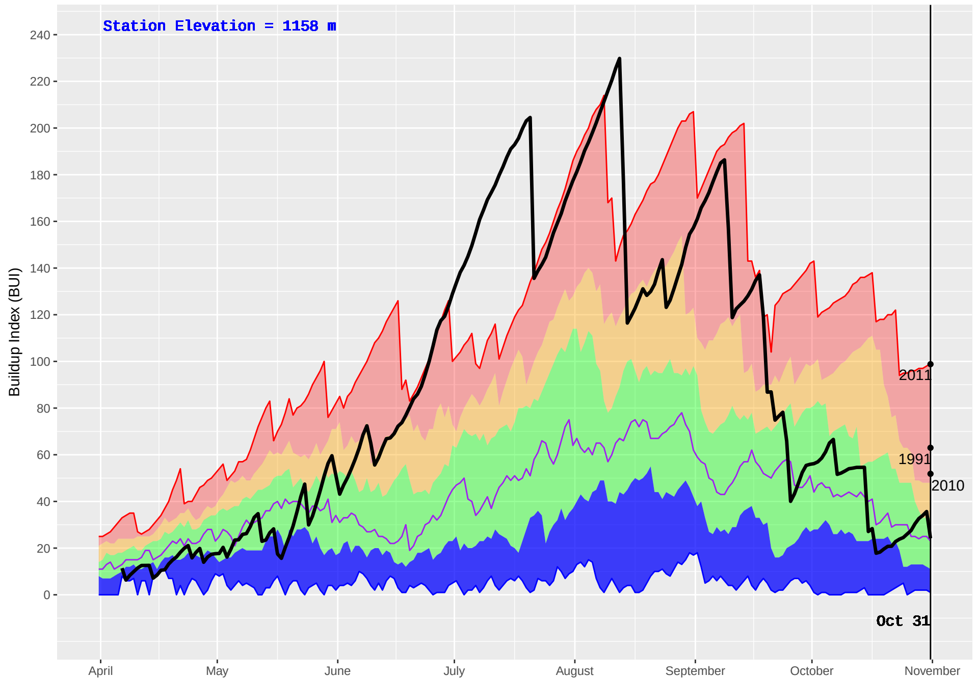
LONE BUTTE (218) : Historical (1987–2016) and Current (2017) Noon Buildup Index (BUI)
